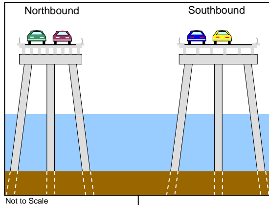
Trestle Cross-section
