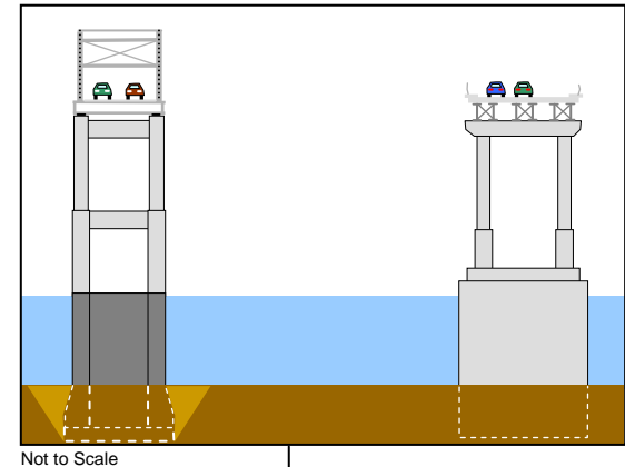
North Channel Bridges Cross-section
