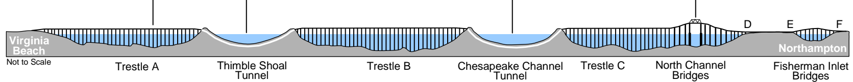
Bridge-Tunnel Profile
